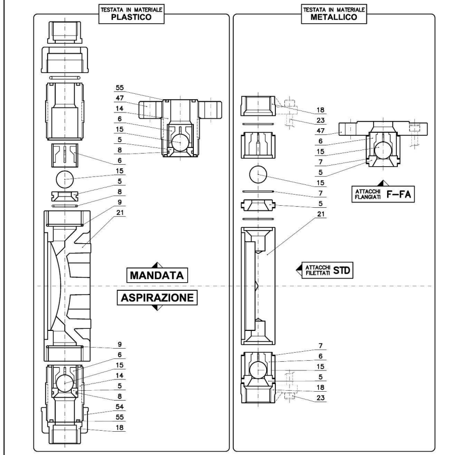
Figure 15 PUMP MODELS M150-M521: PUMP HEAD COMPONENTS (ø165)
